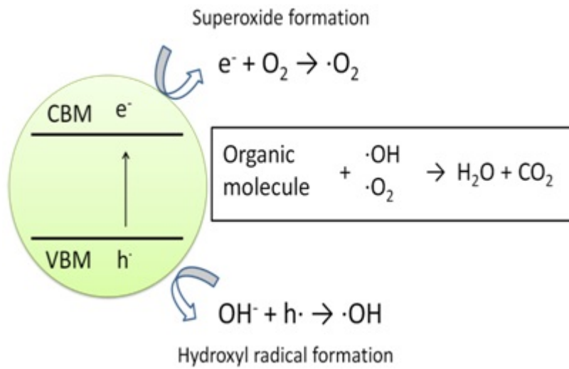
Figure 4. Band diagram and schematics of degradation of organic compounds over a photocatalyst surface [12,33].
